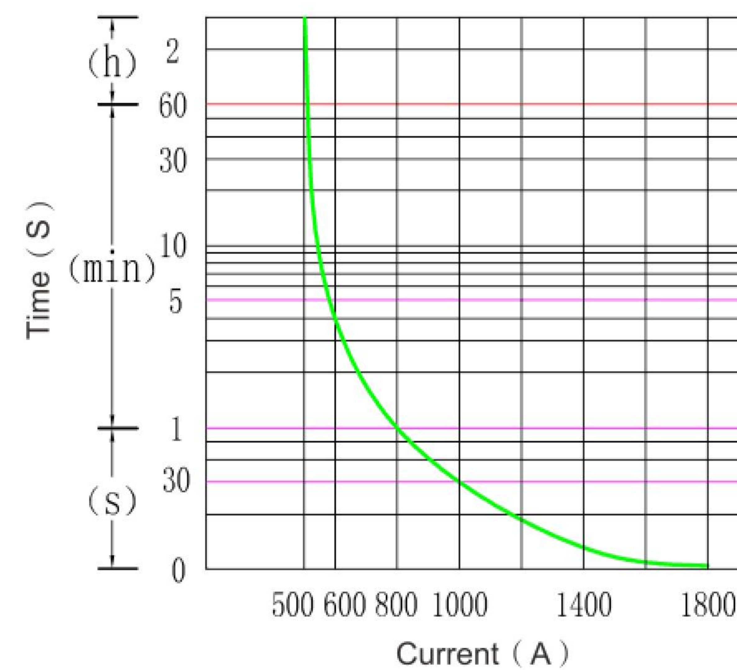
Short overload capacity curve
