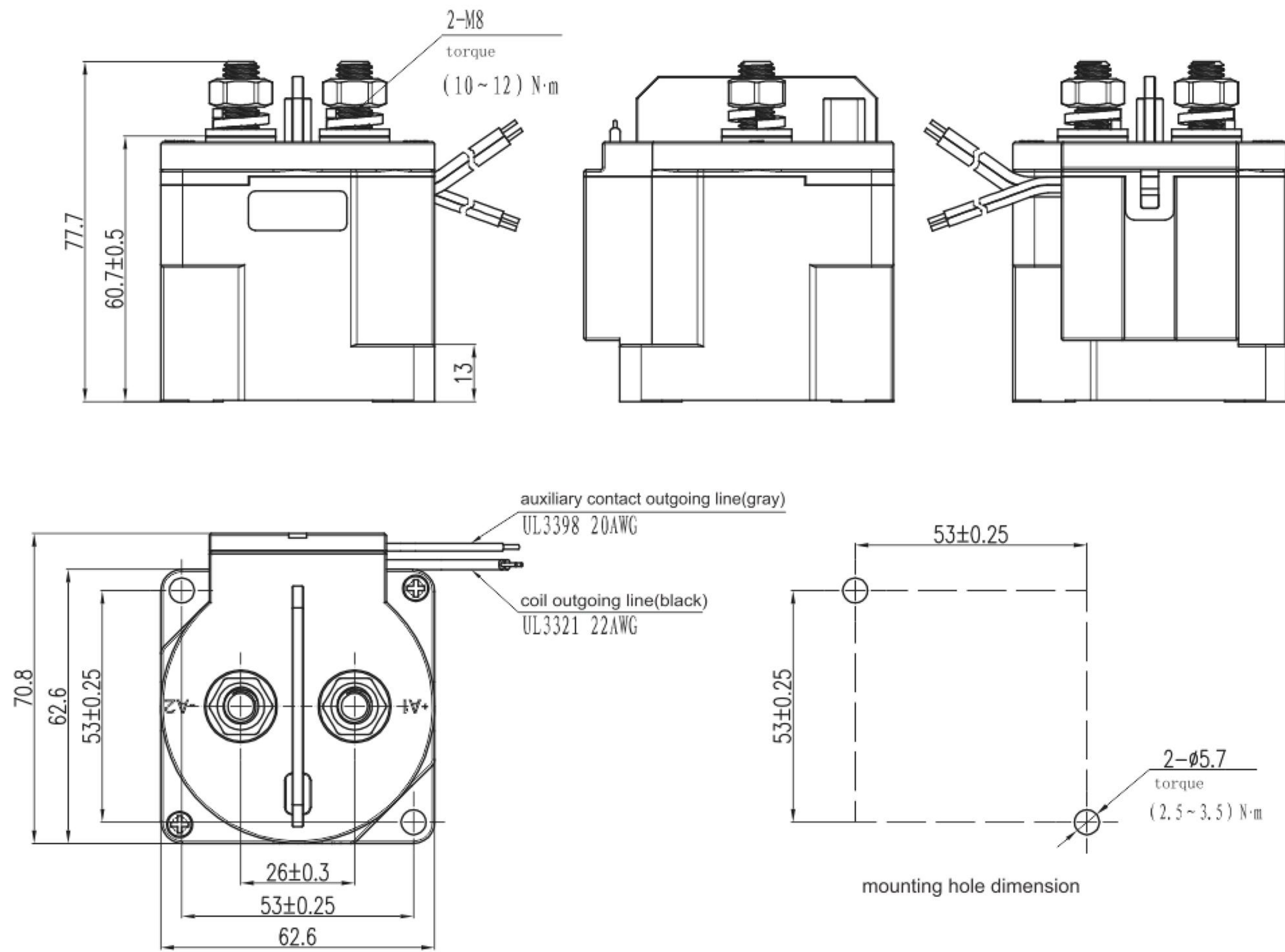
HVC-500 outline dimension
