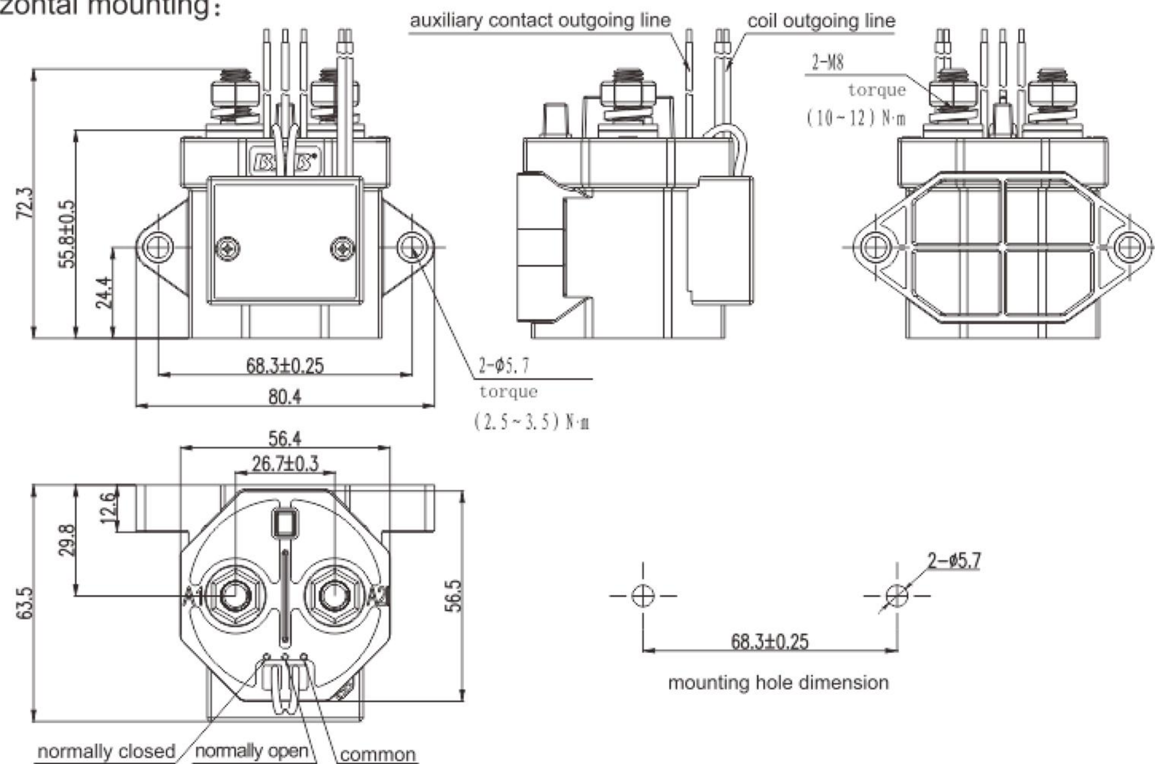
outline dimension
