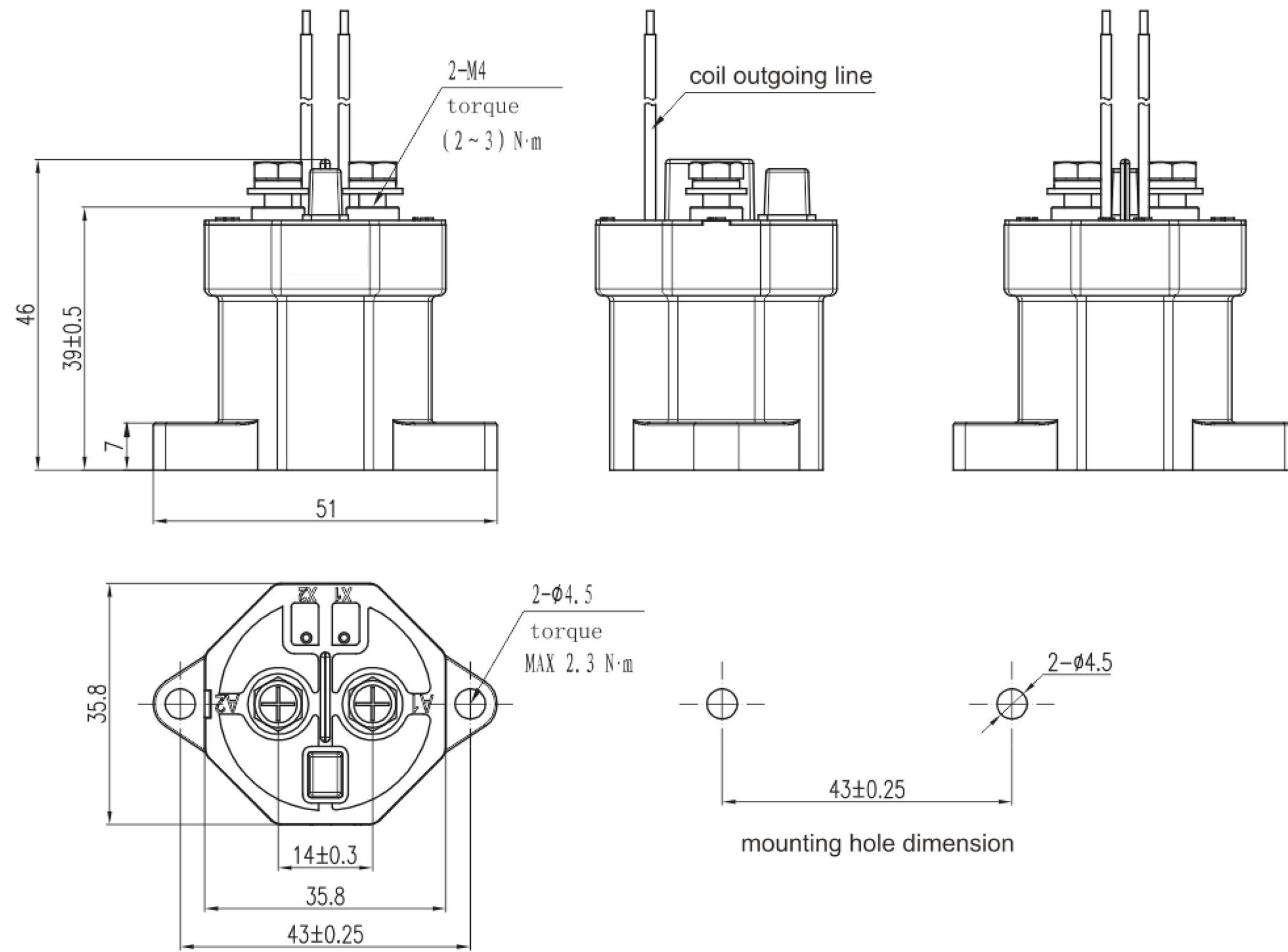
HVC-30 outline dimension
