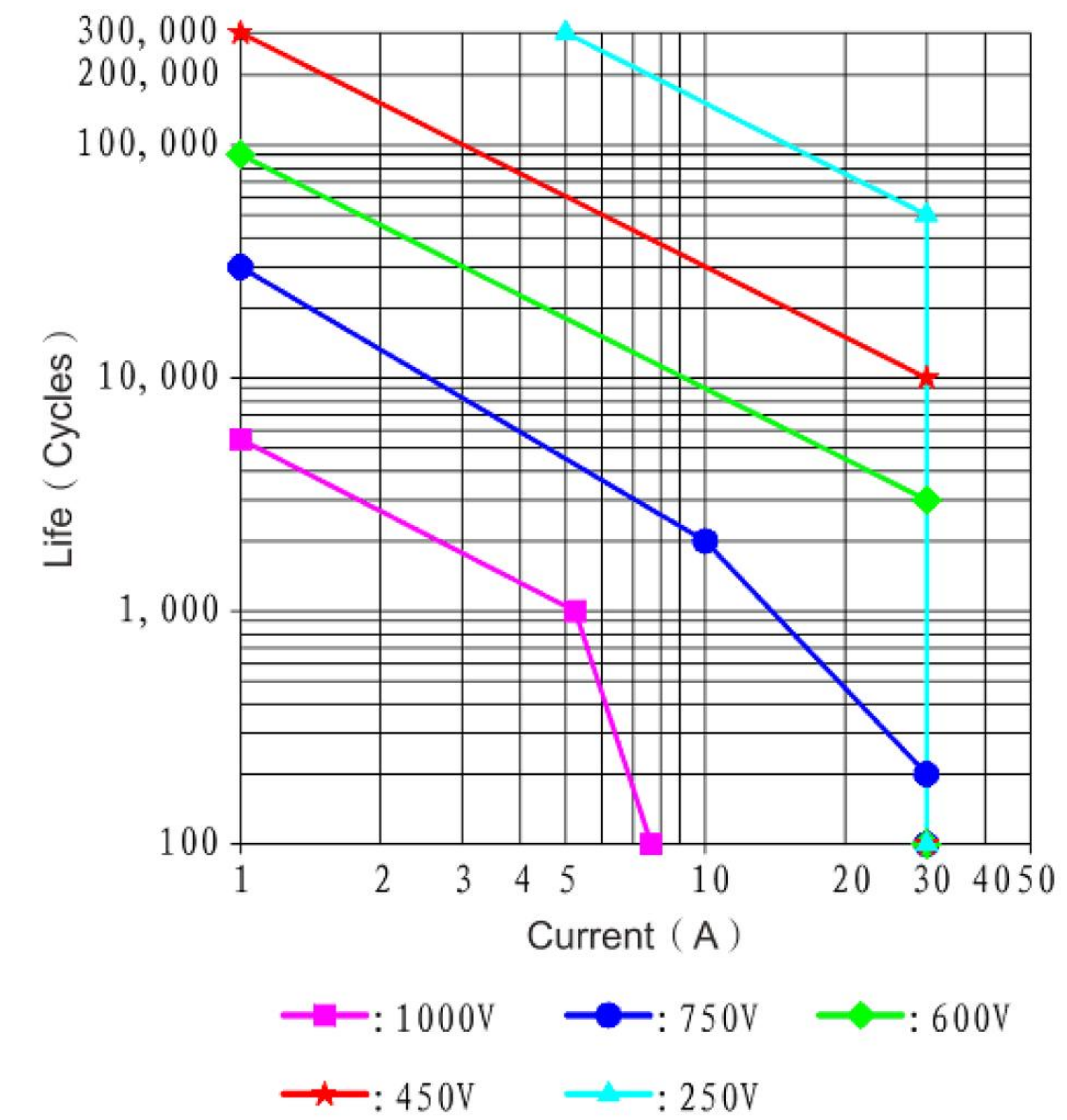
Cut-off life curve of resistive load
