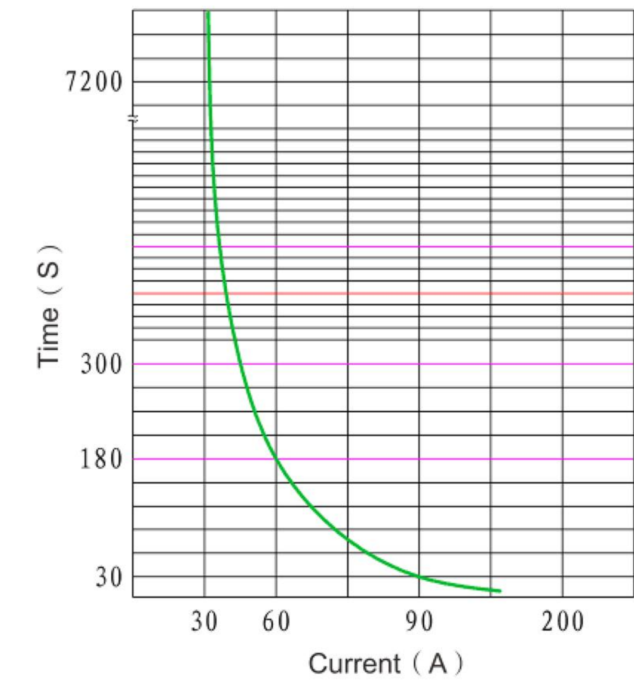
Short overload capacity curve
