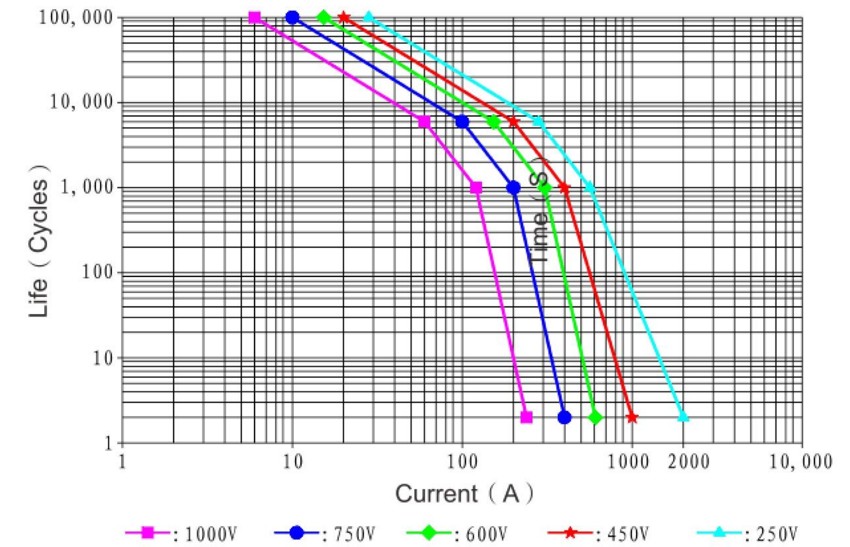
Cut-off life curve of resistive load
