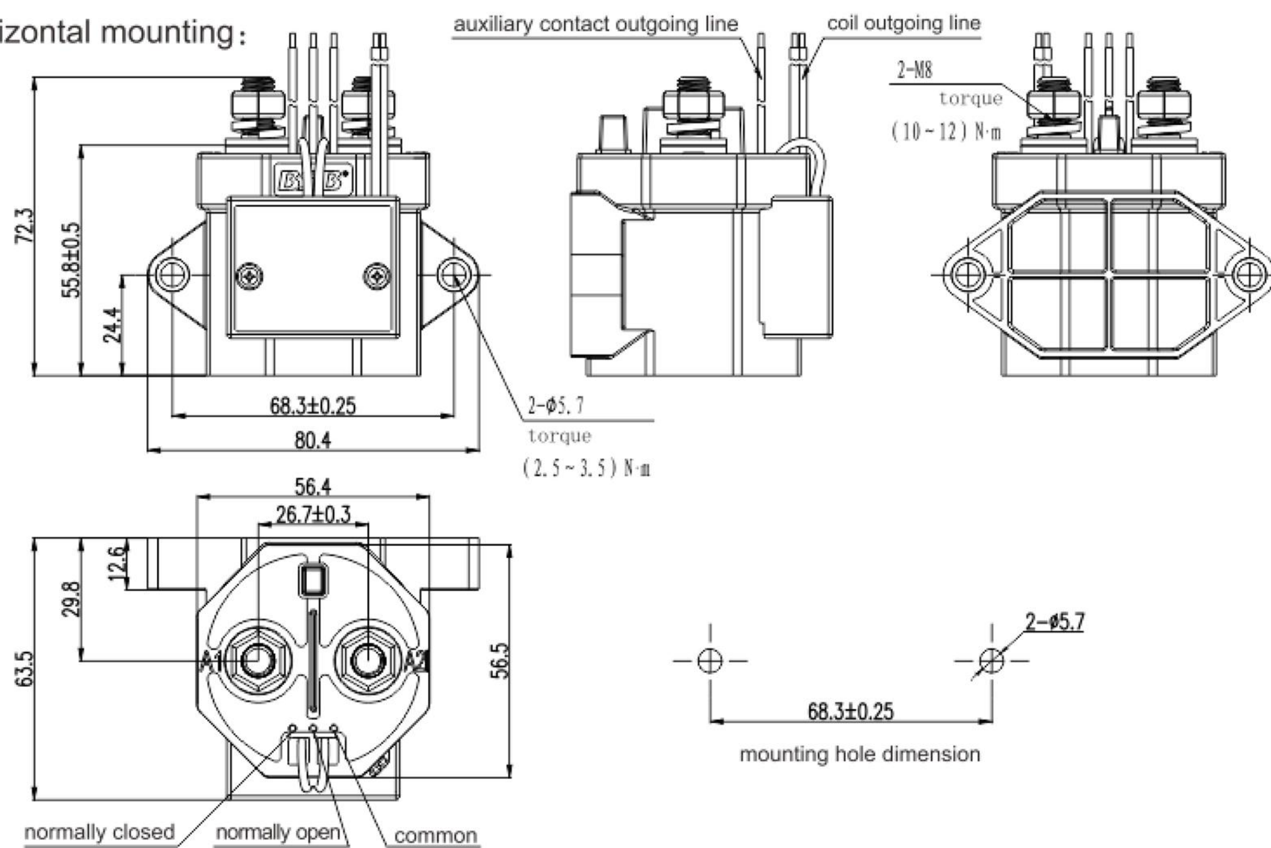
HVC-200 outline dimension
