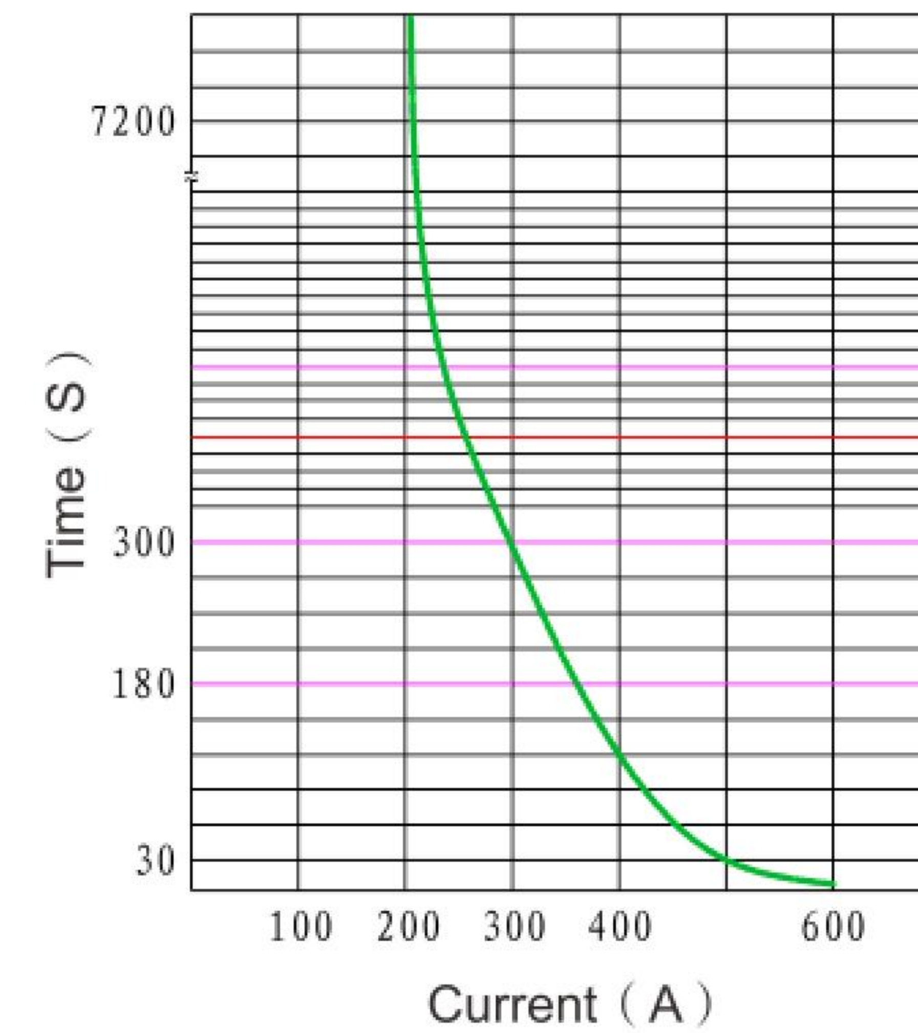
Short overload capacity curve
