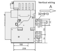
Vertical wiring
