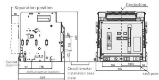
EHW5DC-2500 Drawer type circuit breaker (3 poles)
