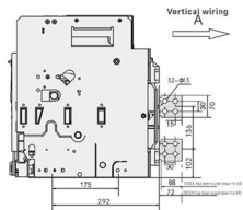
Vertical wiring
